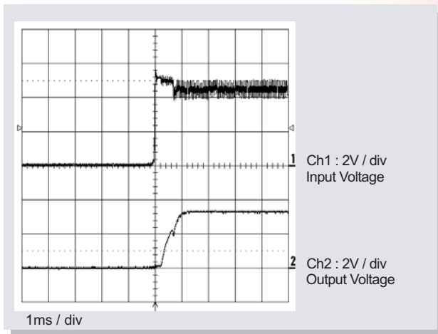
Fig12. Start-up with Application of Vin ( V_o = 3.3V , I_o = 5A )
