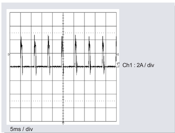
Fig16. Input Current with Short Circuit at Output ( V_o = 3.3V , I_o = 5A )
