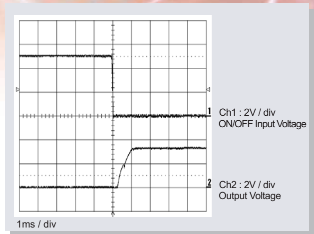
Fig13. Start-up Using Remote ON/OFF with Prebias ( V_o = 3.3V , I_o = 5A )
