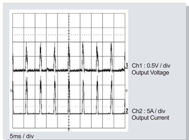
Fig17. Output Current & Voltage with short Circuit at Output ( V_o = 3.3V , I_o = 5A )
