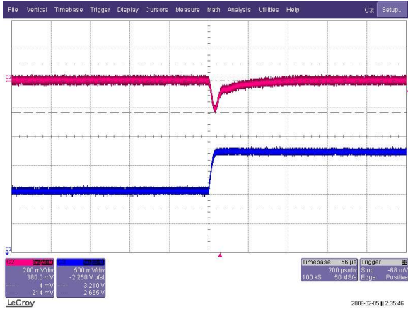
[Fig.22] Load step: 50%-75% of I_o , di/dt=0.1A/us (CH1: 200mV, CH2: 2.5A/div, 200us/div)
