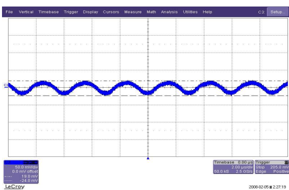
[Fig.26] Input reflect ripple current (250mA/div)
