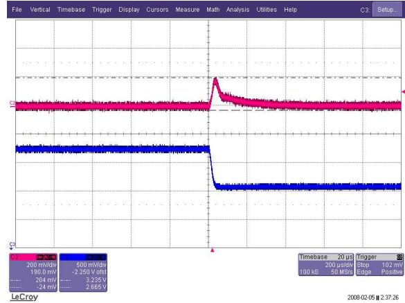
[Fig.23] Load step: 70%-50% of I_o , di/dt=0.1A/us (CH1: 200mV, CH2: 2.5A/div, 200us/div)
