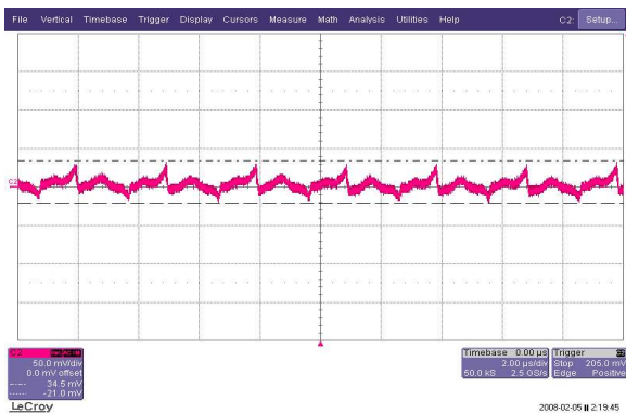
[Fig.24] Output voltage ripple & noise (50mV/div) (1 \mu F ceramic + 15 \mu F tantalum, Bandwidth : 20MHz, See fig.30)
