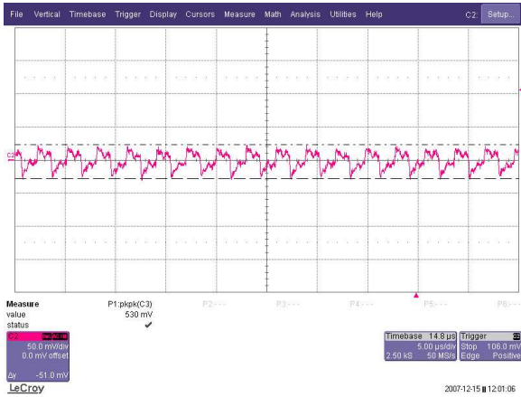
[Fig.15] Output voltage ripple & noise (50mV/div) (1μF ceramic + 15μF tantalum, Bandwidth : 20MHz, See fig.30)
