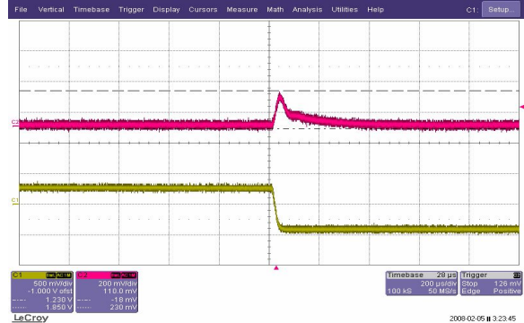
[Fig.23] Load step: 70%-50% of I_o , di/dt=0.1A/\mu s (CH1: 200mV, CH2: 2.5A/div, 200us/div)
