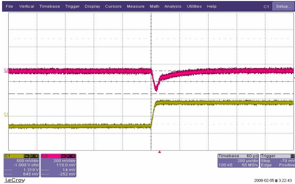
[Fig.22] Load step: 50%-75% of I_o , di/dt=0.1A/\mu s (CH1: 200mV, CH2: 2.5A/div, 200us/div)
