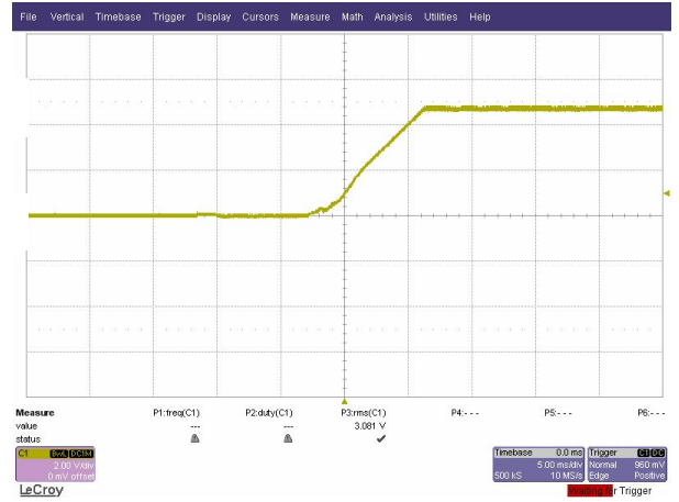
CH1: 2V/DIV 5ms/DIV
