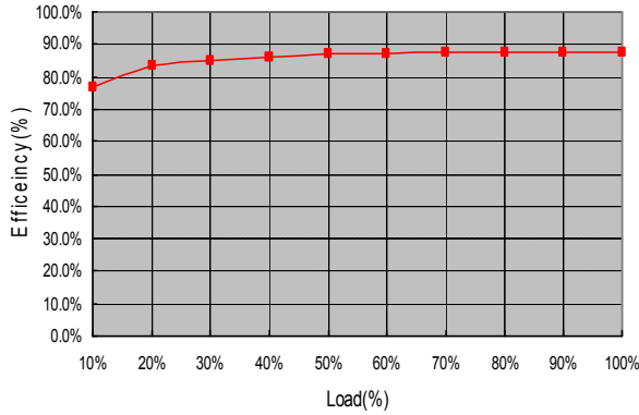
Efficiency curve vs load
