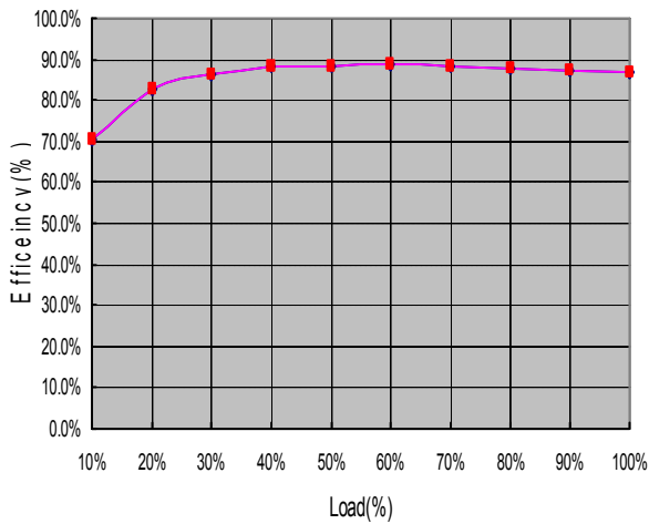
Efficiency curve vs load
