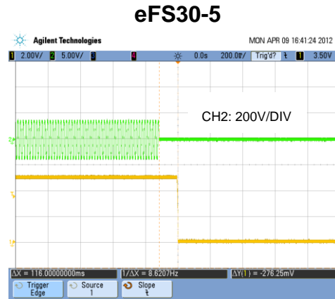
Vin = 220VAC, Vo=5V @6A, At 25°C
