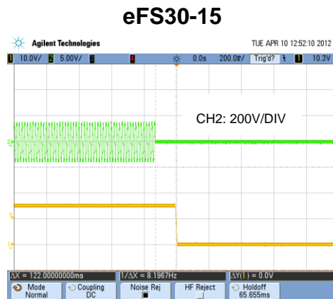
Vin=220VAC, Vo=15V @2A, At 25°C
