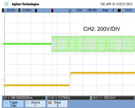
Vin=220VAC, Vo=24V @1.25A, At 25°C
