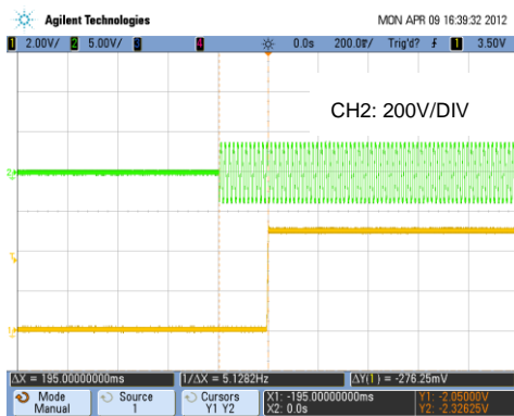
Vin=220VAC, Vo=5V @6A, At 25°C
