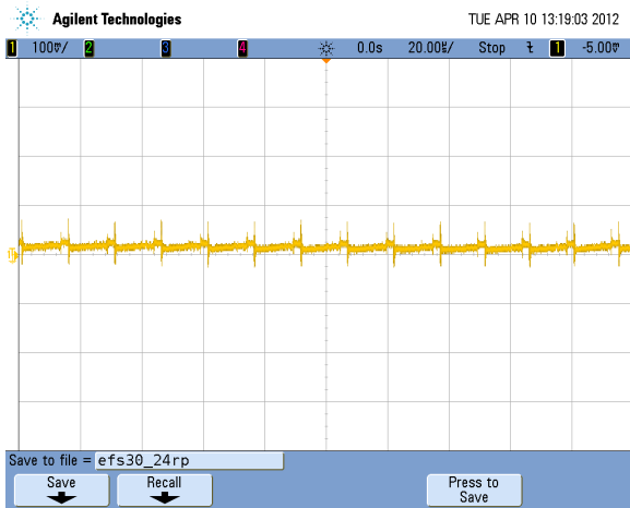
Vin=220VAC, Vo=24V@1.25A, At 25°
