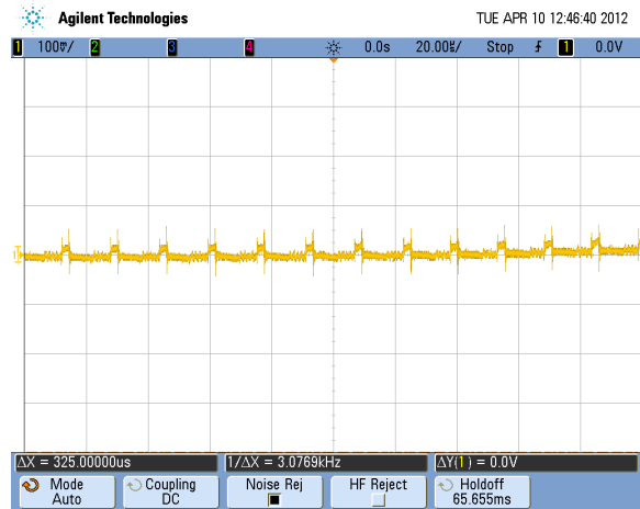
Vin=220VAC, Vo=12V @2.5A , At 25°
