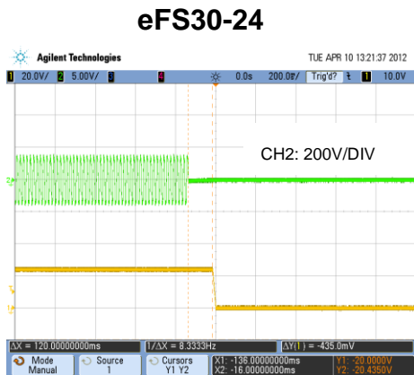
Vin=220VAC, Vo=24V @1.25A , At 25°C
