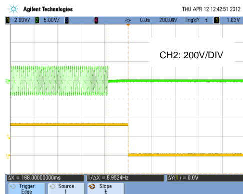
Vin=220VAC, Vo=3.3V @6A, At 25°C
