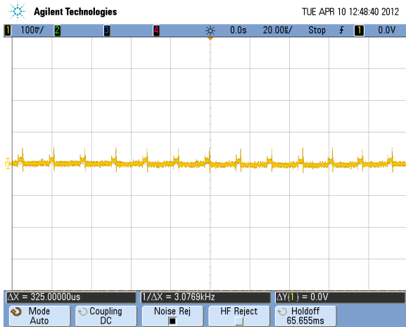
Vin=220VAC, Vo=15V@2A, At 25°
